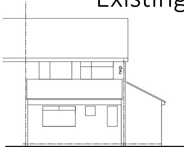
FRONT ELEVATION
